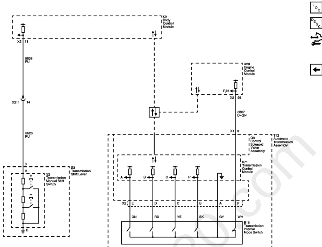
Fig. 3: IMS and Tap Up/Tap Down (MH7 or MHC) Courtesy of GENERAL MOTORS CORP.
